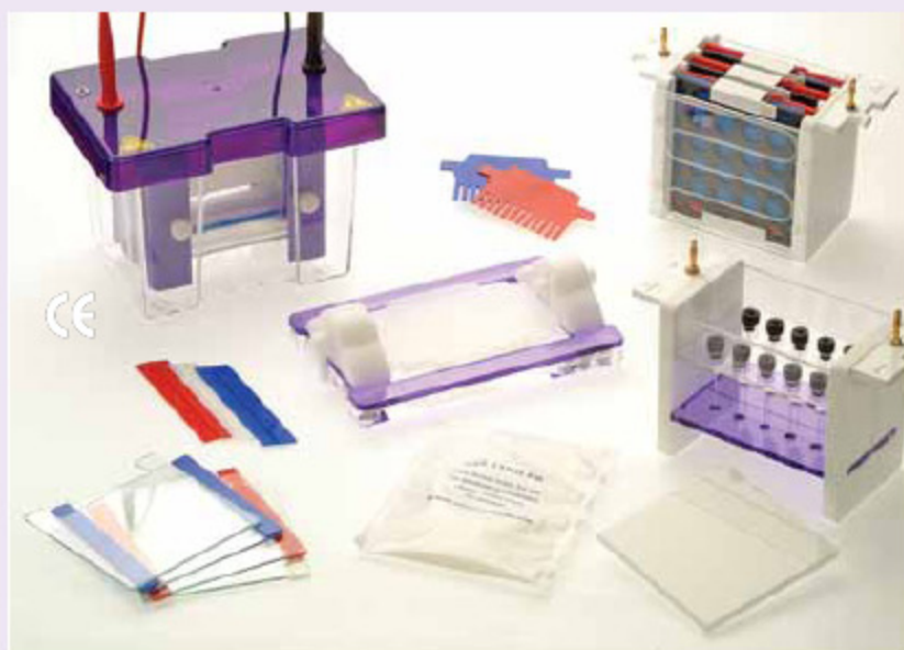
components and accessories of omniPAGE Mini, VS10CES
